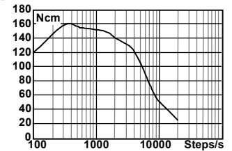
DRIVE: BIP.CHOP., 75 V - 6.7 A/PH
