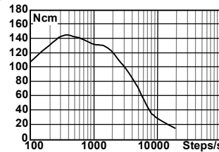
DRIVE: BIP.CHOP. PAR., 75 V - 4.4 A/PH
