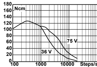
DRIVE: BIP.CHOP. PAR., 2.4 A/PH
