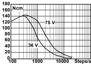
DRIVE: BIP.CHOP. PAR., 1.8 A/PH
